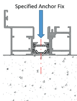
Typical outer frame installation
